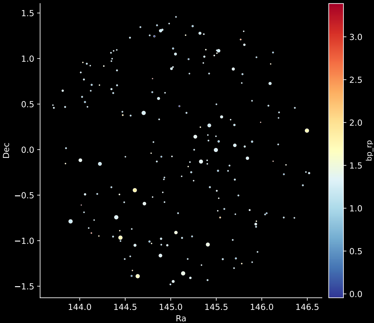
APOGEE DR17 Field: [177-49_MGA] Stars: 198
