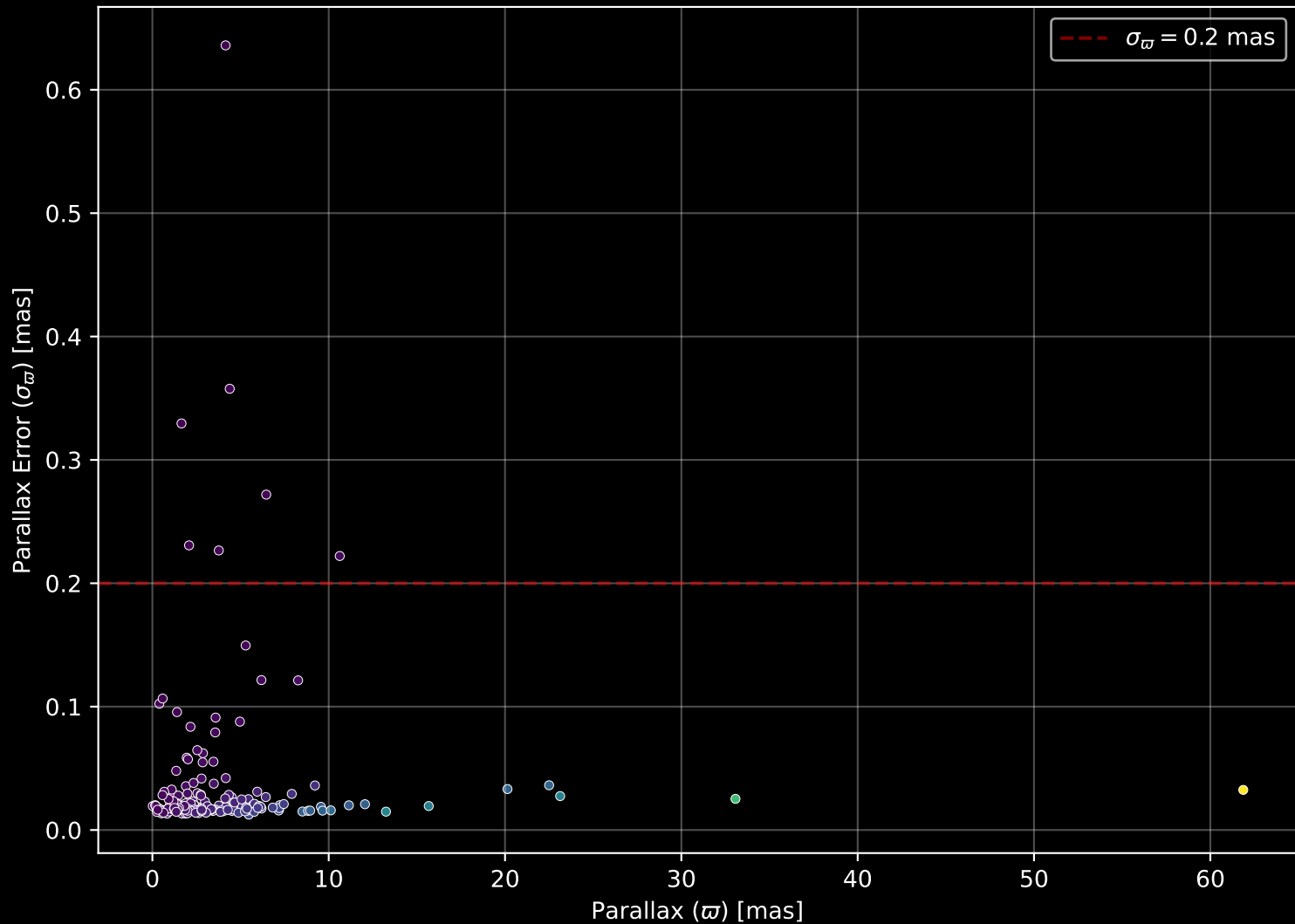
APOGEE DR17 Field: [177-49_MGA] Parallax Quality (n= 198)
