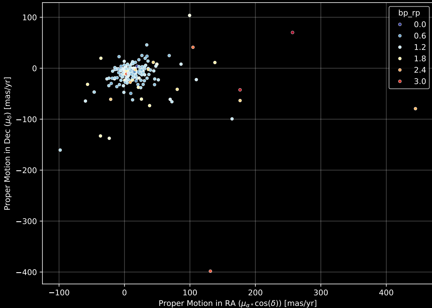
APOGEE DR17 Field: [177-49_MGA] Proper Motion Diagram (n= 198)
