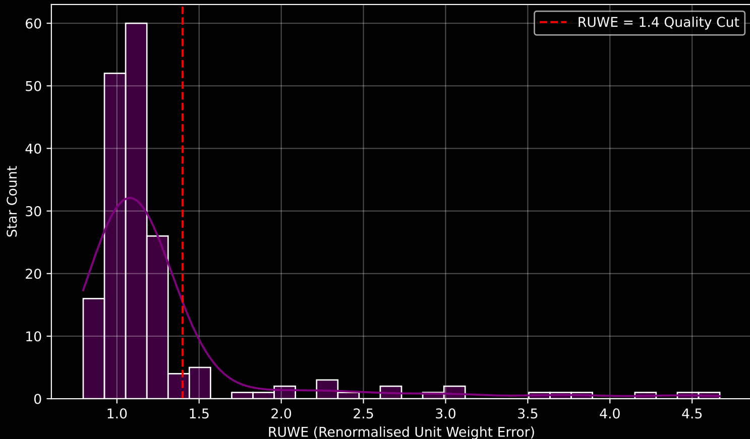
GAPOGEE DR17 Field [177-49_MGA] RUWE Distribution (n= 182)
