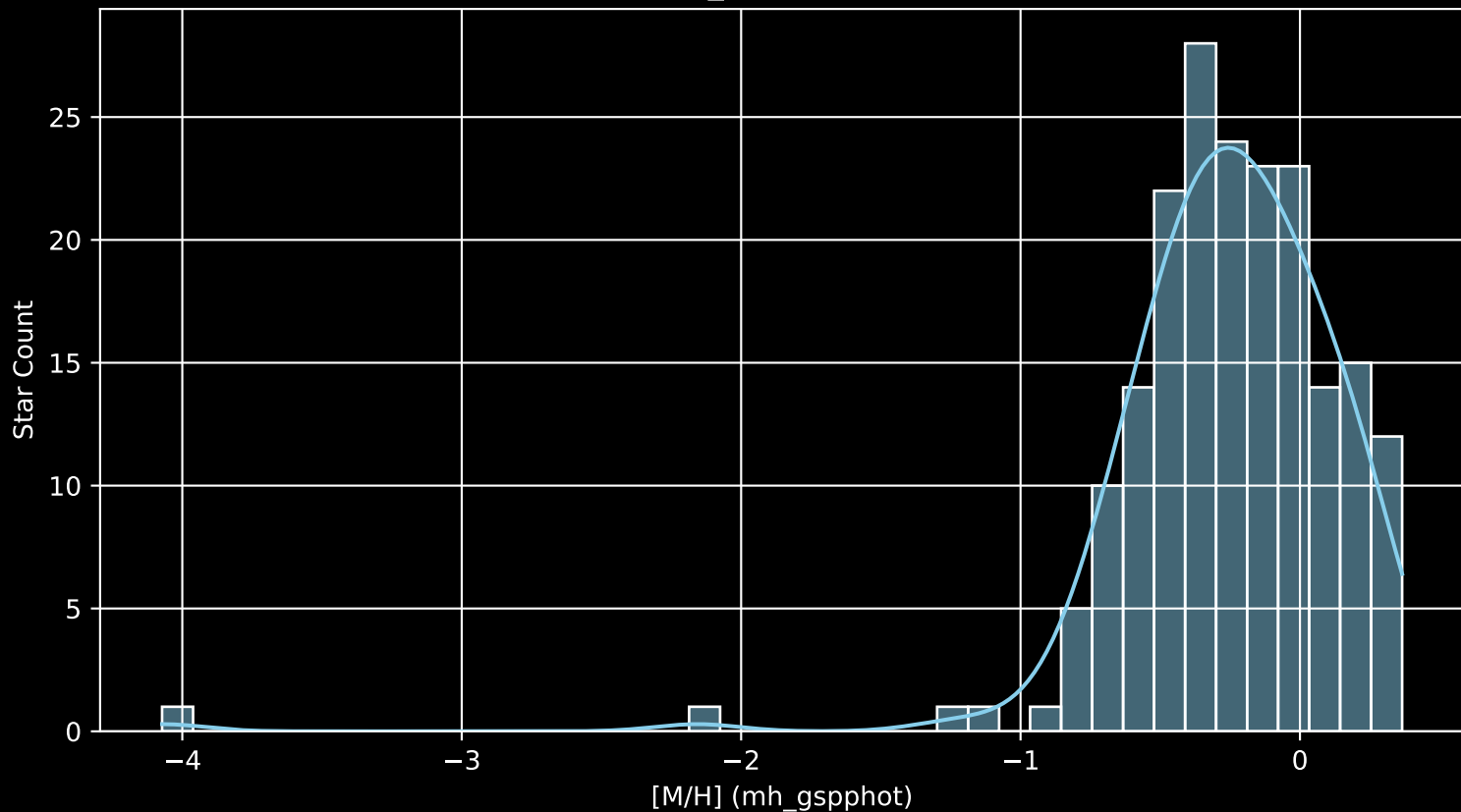
APOGEE DR17 Field: [177-49_MGA [M/H] (mh_gspphot) (n= 195)
