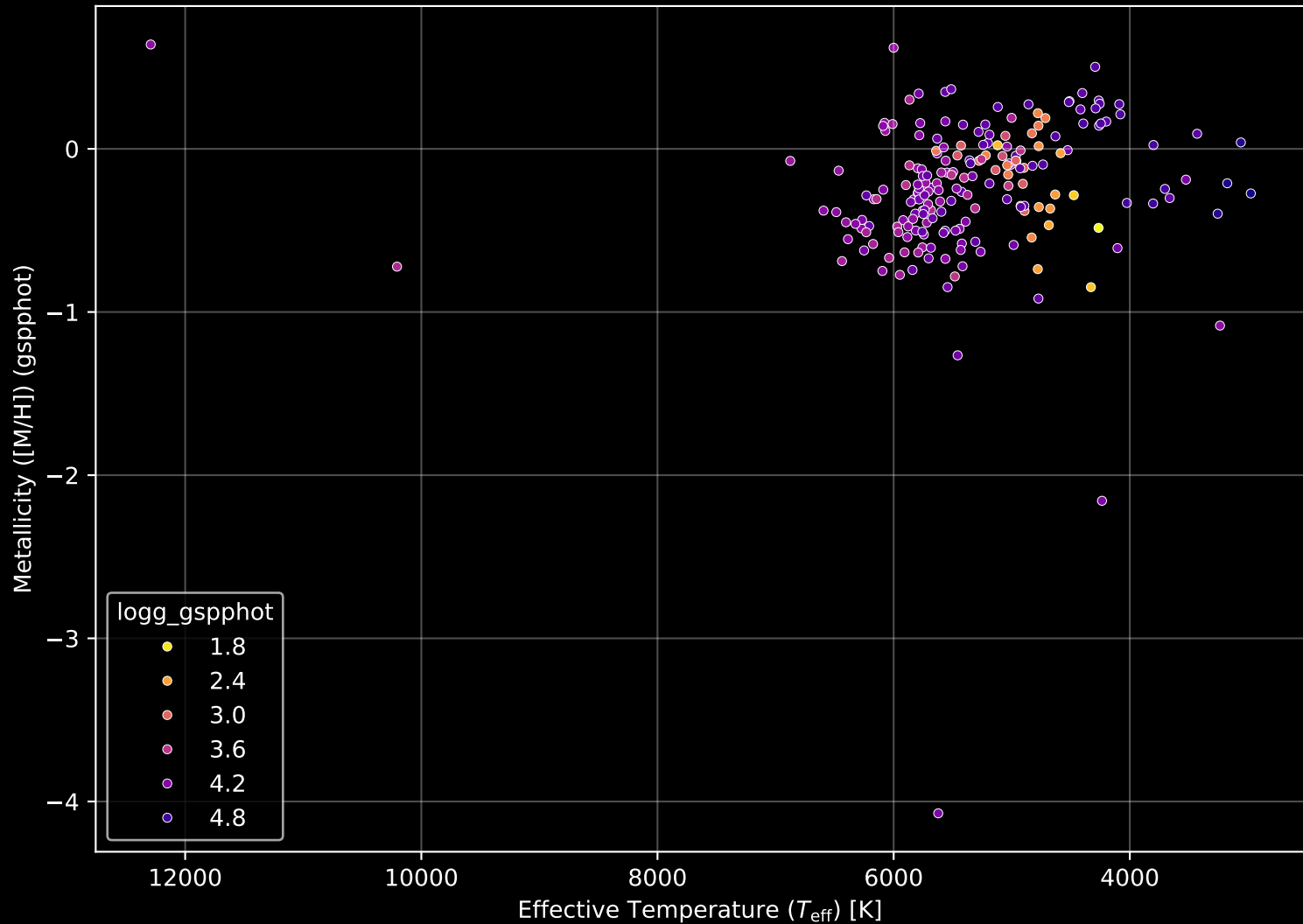
APOGEE DR17 Field: [177-49_MGA] Stellar Population Parameters (n= 198)
